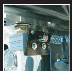
Carriage-Hydraulic Placement
